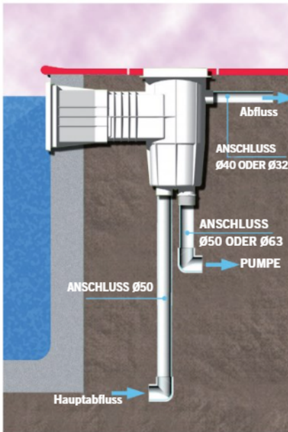
INSTALLATION SKIMMER
